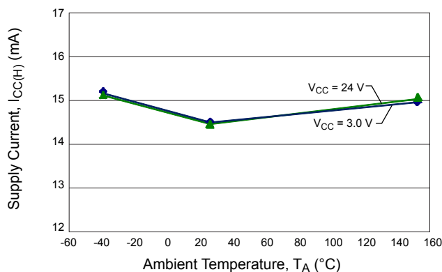
Average Supply Current (High) versus Temperature
