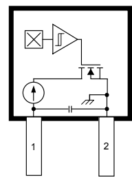
Pinout Diagram
