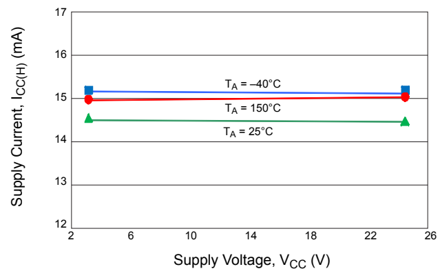
Average Supply Current (High) versus Supply Voltage
