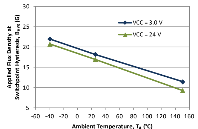
Average Switchpoint Hysteresis versus Temperature
