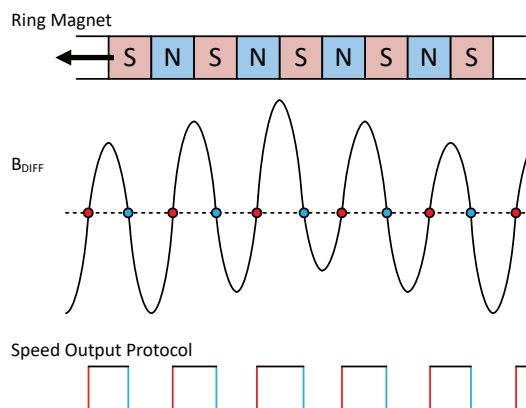
Figure 7: Fixed Threshold Option Switch Point Algorithm
