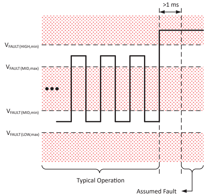
Figure 11: Assumed Fault Example: High Fault
