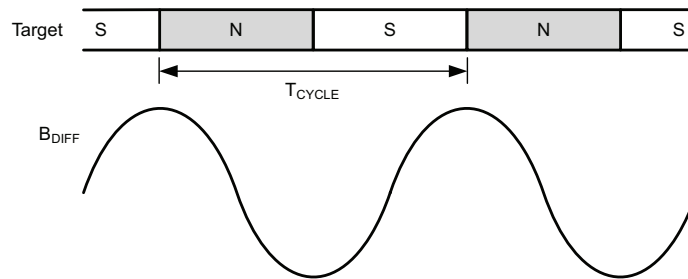
Figure 1: Definition of T_{\text{CYCLE}}
