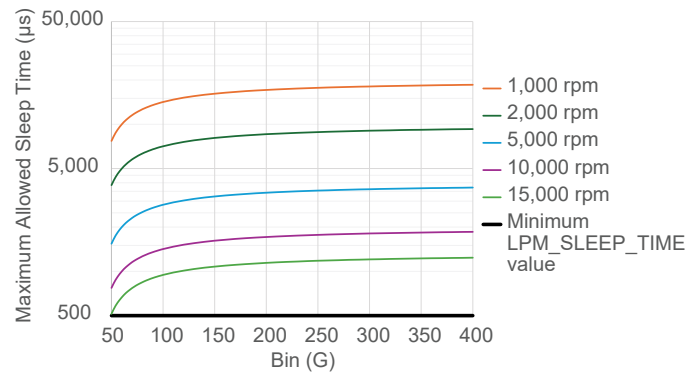
Figure 22: Maximum Allowed Sleep Time vs. Bin vs. Maximum Target Rotation Speed
