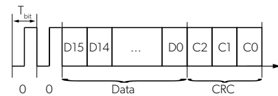
Figure 40: Manchester Read Acknowledge Command
