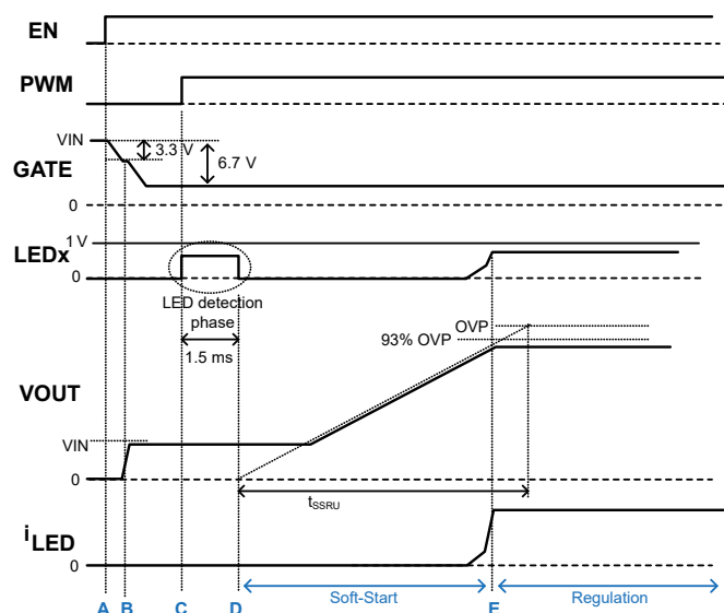
Figure 9: Complete startup process of A80602
