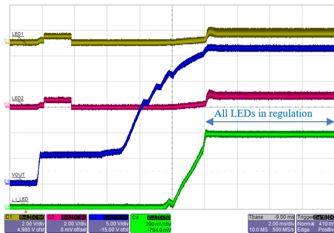
Figure 32: A80602 Normal startup sequence showing voltage at LED1 and LED2 pins. V_{IN} = 6V , output = 8 \times WLED in series, current = 6 \times 100mA
