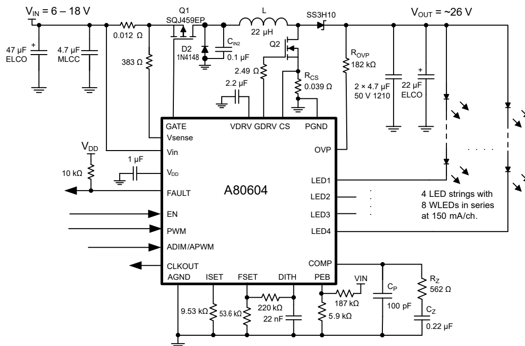
Figure 52: Boost Design Example Schematic ( f_{SW} = 400 kHz)
