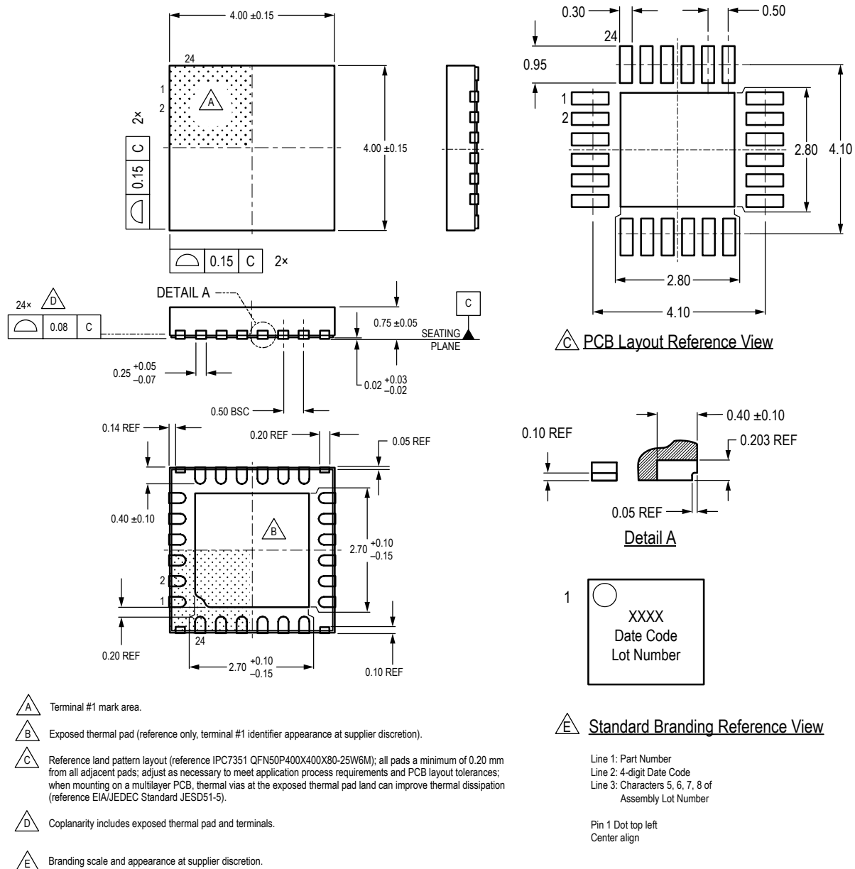
Figure 49: Package ES, 24-Pin 4 mm x 4 mm QFN with Exposed Thermal Pad and Wettable Flank
