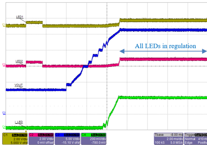
Figure 37: A80604 Normal startup sequence showing voltage at LED1 and LED2 pins. V_{IN} = 6V , output = 8 \times WLED in series, current = 4 \times 100mA
