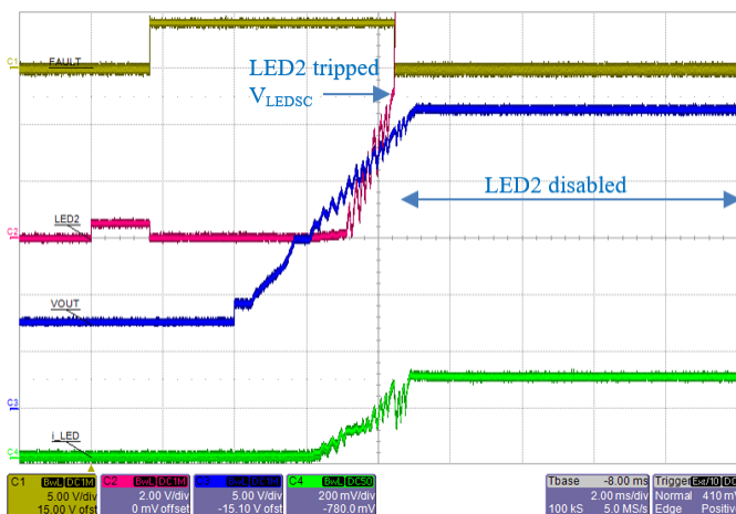
Figure 38: A80604 startup sequence when LED string#2 has a partial-short fault ( 6 \times WLED instead of 8). As soon as LED2 pin rises above V_{LEDSC} (~5 V), the channel is disabled and FAULT = Low . All other channels continue as normal.
