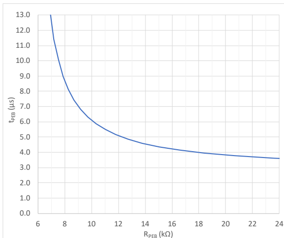
Figure 20: How PEB delay time varies with value of PEB pin resistor to GND.
