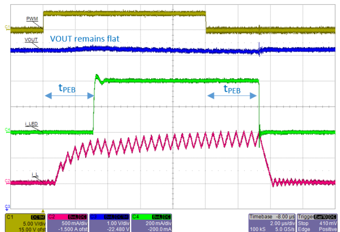
Figure 19: A80605 PWM dimming operation with PEB delay set to 3 \mu s. Note that V_{OUT} ripple is reduced to ~0.2 V.
