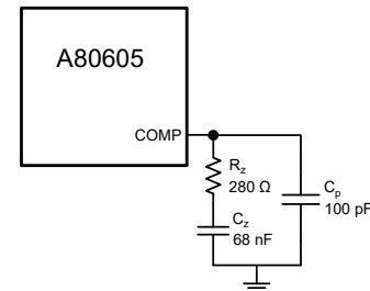
Figure 47: Compensation Network Schematic
