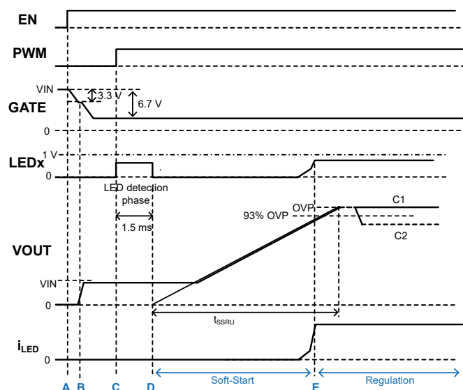
Figure 9: Complete startup process of A80606
