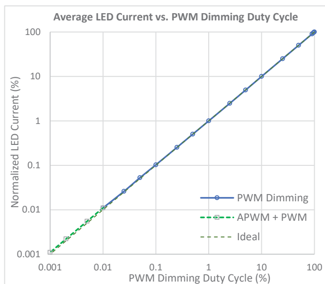
Figure 29: How to achieve 100,000:1 dimming ratio by using both PWM and APWM. Test conditions: V_{\text{IN}} = 12 \text{ V} , V_{\text{OUT}} = 25 \text{ V} ( 8 \times \text{WLED} ), total LED current = 400 mA, PWM frequency = 200 Hz, APWM frequency = 100 kHz.
