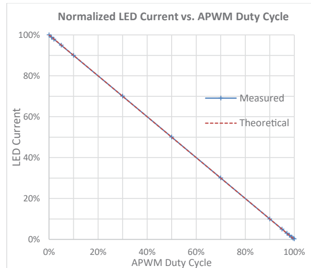
Figure 26: Showing LED current is inversely proportional to the APWM duty cycle. Test conditions: V_{IN} = 12 V, V_{OUT} = 25 V ( 8 \times WLED), total LED current = 100 \text{ mA} \times 4 , APWM frequency = 100 kHz
