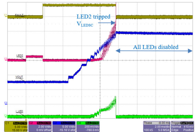
Figure 39: A80606-1 startup sequence when LED string#2 has a partial-short fault ( 6 \times \text{WLED} instead of 8). As soon as LED2 pin rises above V_{LEDSD} ( \sim 5\text{ V} ), all channels are disabled and \text{FAULT} = \text{Low} .
