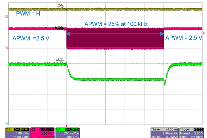
Figure 27: PWM = H. Total LED current drops from 400 mA ( 4 \times 100 \text{ mA/ch} ) to 300 mA when APWM of 25% duty cycle is applied. Note that LED current takes ~1 ms to settle after change in APWM.
