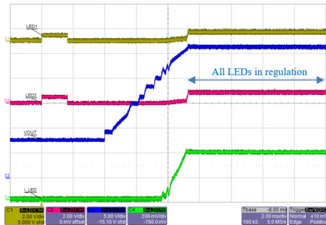
Figure 37: A80606 Normal startup sequence showing voltage at LED1 and LED2 pins. V_{IN} = 6\text{ V} , output = 8 \times \text{WLED} in series, current = 4 \times 100\text{ mA}
