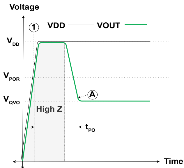
Figure 7: Power-On Delay, t_{PO}
